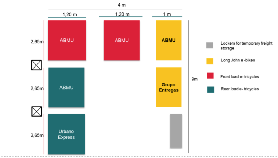
Fig 6. Cross docking vehicles distribution
